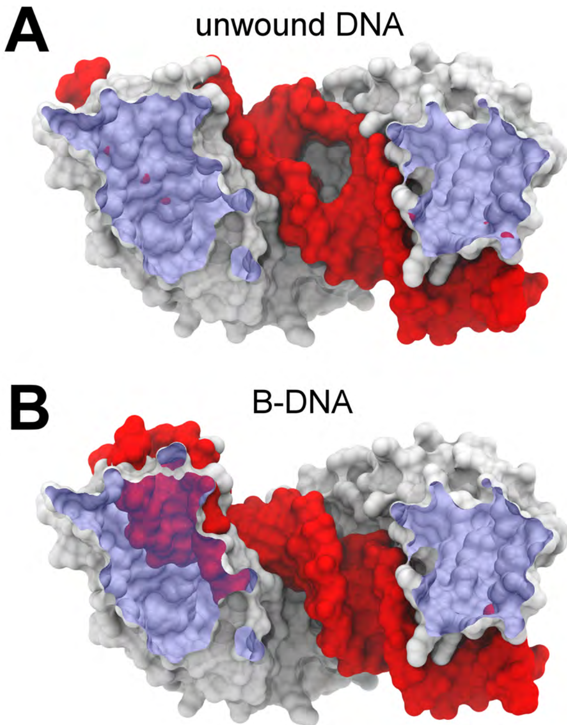
Figure 5.9. MTERF1 in the recognition mode conformation is too unwound to track the major groove of B-DNA. Surfaces were sliced to show incompatibility: the blue clipping plane appears purple where the DNA penetrates the protein. (A) Only minor steric clashes are present in the crystal structure of the recognition complex with unwound DNA. (B) Aligning the C-site P atoms of B-DNA to the corresponding region in the crystal led to large steric clashes between the N-site and the N-terminal domain of MTERF1. Alignment of the N-site resulted in similar clashes in the C-site.
