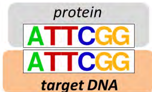
Figure 2.1 Direct readout described by information theory: A regulatory protein (grey) recognizes one specific DNA sequence. (a) The protein can bind any six-letter DNA sequence ( X=A, T, C, G ). The maximum information that can be gained ( \Omega_{\text{seq}} ) depends on the number of possible six-letter sequences. (b) The protein binds a wrong sequence. \Omega_{\text{read}} is maximum. No information is gained ( \Delta\Omega=0 ). (c) The protein binds the target sequence, the \Omega_{\text{read}} is 0. Maximum information is gained ( \Delta\Omega=\text{max} ).
