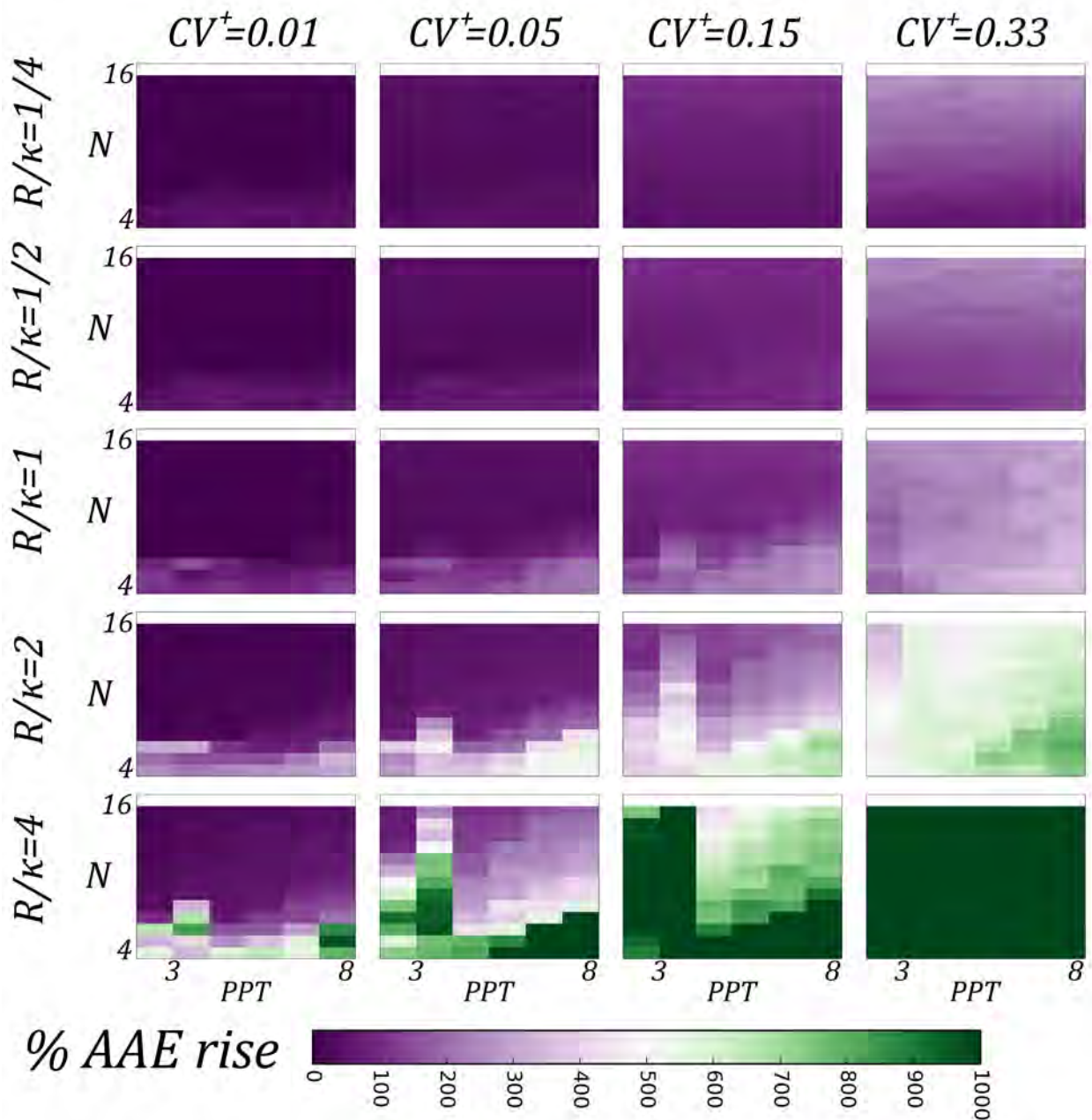
Figure 3.10. Percent AAE of derived helix rise for the 399,360 test helices. Helix matrices are organized per Figure 3.3 . The plotted range of the percent average absolute error is 0 to 1000.
