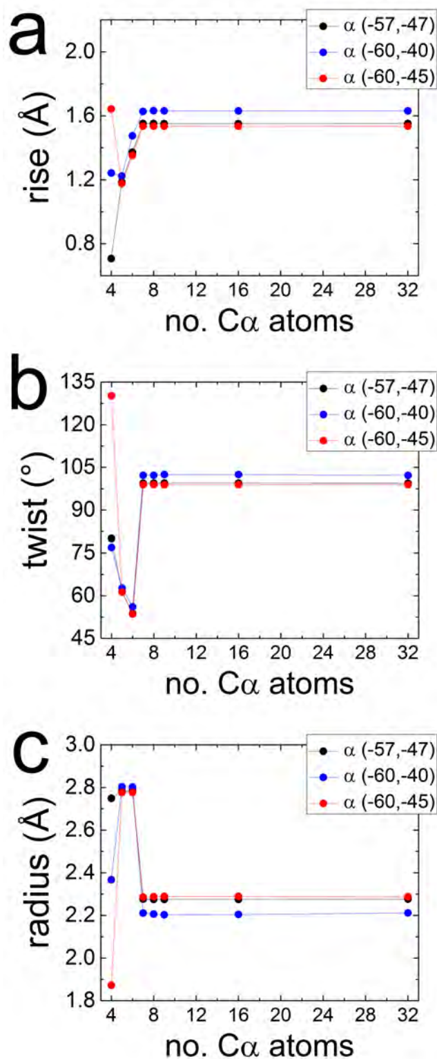
Figure 3.11. Helical parameters of \alpha -helical secondary structure elements defined using three different pairs of \phi/\psi backbone torsions (black, blue and red symbols represent \alpha_{-57,-47} , \alpha_{-60,-40} and \alpha_{-60,-45} respectively), and an increasing number of C \alpha atoms used in the fitting (X axis). Shown on the Y axes are the derived values for (a) rise; (b) twist; (c) radius.
