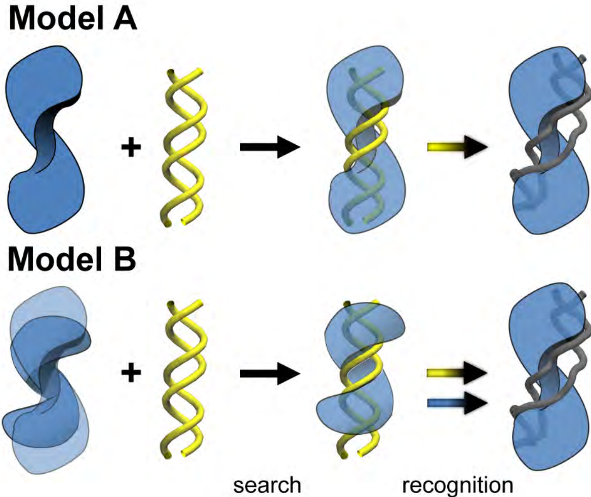
Figure 5.3. Potential MTERF1-DNA binding and recognition mechanisms. Pre-existing unwound DNA that MTERF1 can bind is not likely a viable mechanism (see text). We consider models with either singly or doubly induced fit. Model A: MTERF1 (blue) undergoes minimal conformational adaptation during binding and recognition, with the structure of apo MTERF1, MTERF1 in search mode (nonspecific complex) bound to B-DNA (yellow), and MTERF1 in recognition mode bound to unwound DNA (grey) all being similar in structure. During recognition, only the DNA undergoes conformational change (yellow arrow). Model B: apo MTERF1 is flexible, sampling a diverse ensemble of structures including those with a helical topology similar to B-DNA. During doubly induced fit recognition both MTERF1 and DNA undergo conformational change, blue and yellow arrows, respectively.
