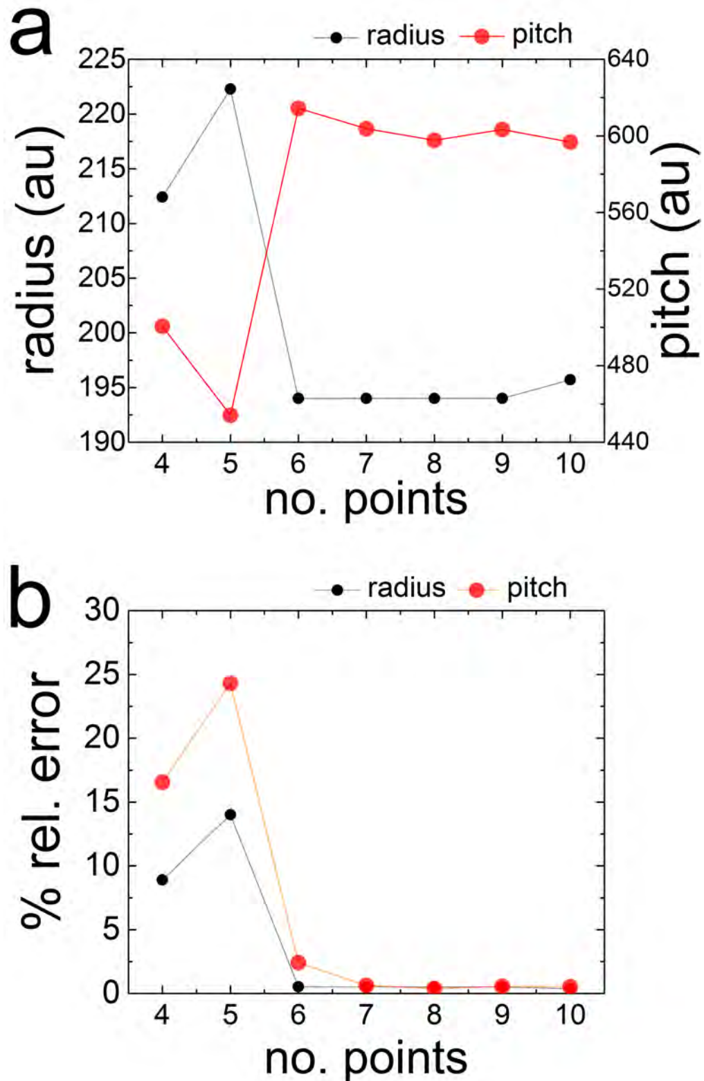
Figure 3.4. Helix parameters of Nievergelt's helix. (a) Helix pitch and radius, with increasing number of points. (b) Percent relative error, using Nievergelt's data as the reference, with increasing number of points.
