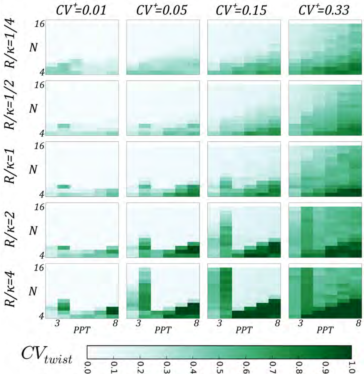
Figure 3.7. Twenty heat-maps of derived CV_{twist} for noisy helices with diverse geometries. Families of helices with five radius-pitch ratios, R/\kappa , are shown, each of which contains a matrix of helices with varying points/turn, PPT , and varying numbers of points, N . For a given N , increasing PPT decreases the number of turns present. For each shape geometry (colored cells, e.g. R/\kappa = 1/4 , CV^+ = 0.01 , N = 16 , PPT = 3 , the top left-most cell), 256 irregular helices were generated subject to Cartesian coordinate perturbations with CV^+ , 0.01, 0.05, 0.15 and 0.33. If a cell in a helix-matrix is light-colored (white), the measured CV_{twist} is low and the method precisely characterizes helix twist. However, if a cell is dark-colored (green), the measured CV_{twist} is large and the method does not precisely characterize helix twist; the method is susceptible to noise.
