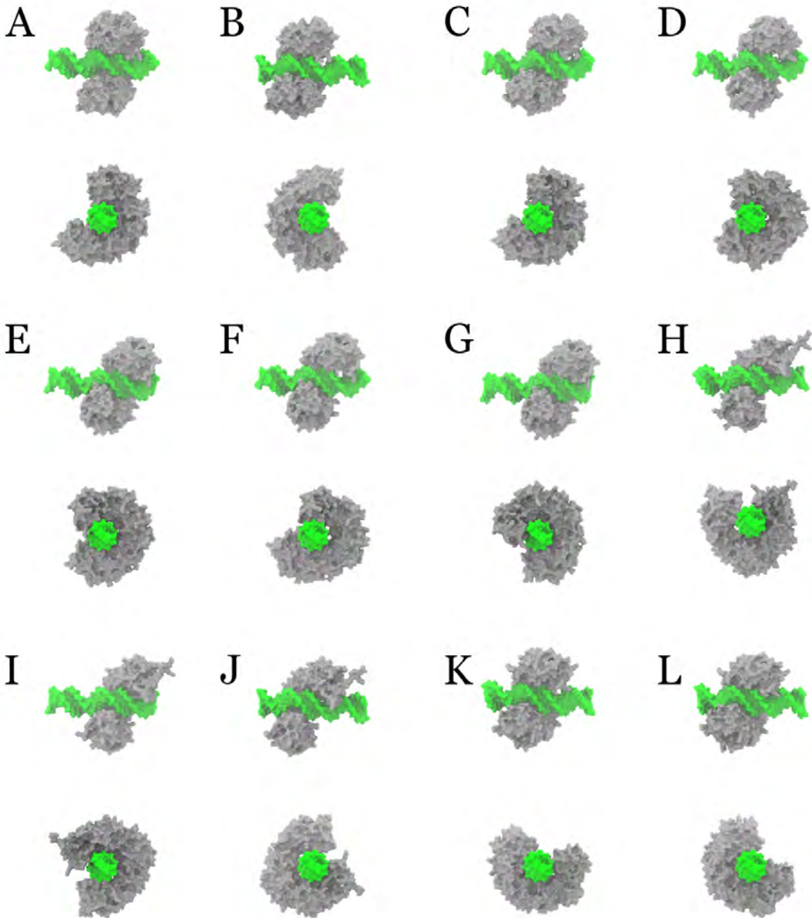
Figure 5.15. The 12 models of the nonspecific complex that best track the major groove obtained by docking low-pitch apo MTERF1 structures to B-DNA. The protein conformations that were used to generate the pose has the following helical parameters (pitch, radius, sweep): for (A) and (B): 41.1 Å, 9.8 Å, 372°; for (C): 41.6 Å, 10.1 Å, 368°; for (D), (E), (F) and (G): 40.3 Å, 11.4 Å, 340°; for (H) and (I): 39.8 Å, 16.2 Å, 276°; for (J): 37.8 Å, 16.0 Å, 287°; for (K) and (L): 34.5 Å, 9.8 Å, 389°.
