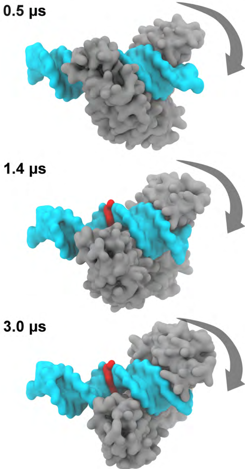
Figure 5.19. Snapshots of the complex at different time points. MTERF1 is shown in grey and is shown DNA in aqua, with the central bp colored red to visually highlight MTERF1 translocation along the major groove of B-DNA. Snapshots are RMS aligned to only the DNA backbone so that MTERF1 is seen to move (rightward) with respect to the DNA frame (indicated by arrows).
