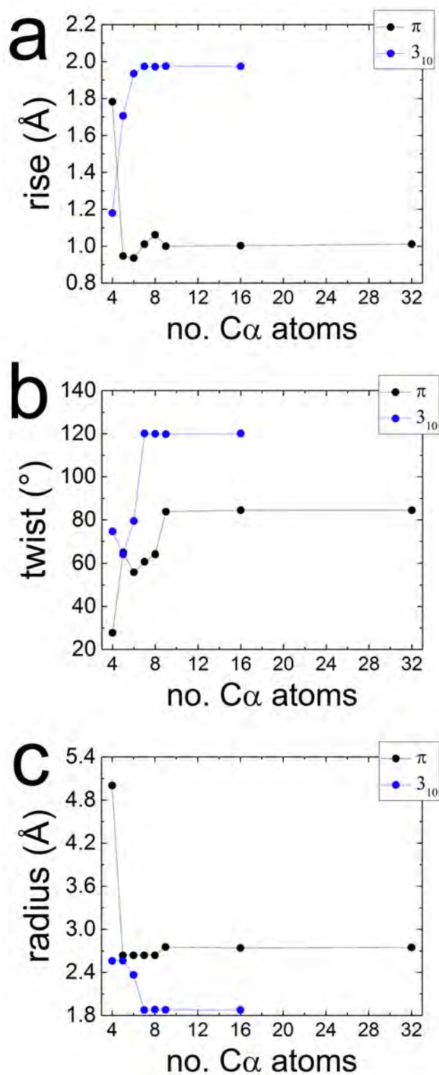
Figure 3.13. Helical parameters of \pi - and 3_{10} - helical secondary structure elements, black and blue symbols respectively, with an increasing number of C \alpha atoms used in the fitting (X axis). Shown on the Y axes are the derived values for (a) rise; (b) twist; (c) radius.
